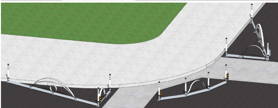
SAMPLE LAYOUT #2: CURB EXTENSION
